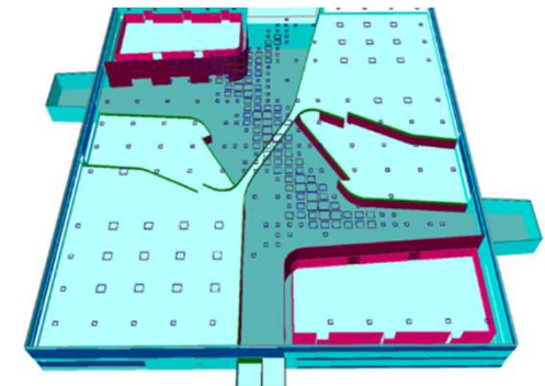
BMW New Car Production Plant , Shenyang (China), Energetic optimization of central building, 3 D Simulation
